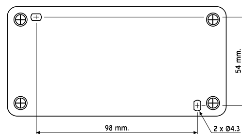
Mounting holes
