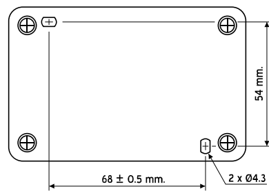
Mounting holes
